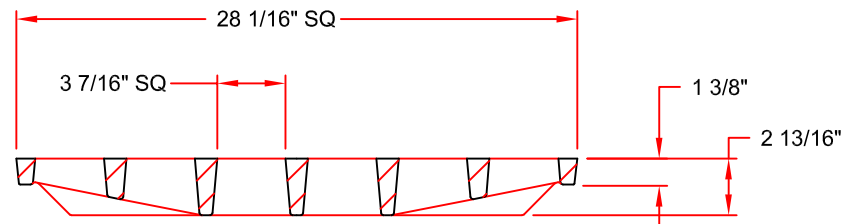
GRATE SECTION
