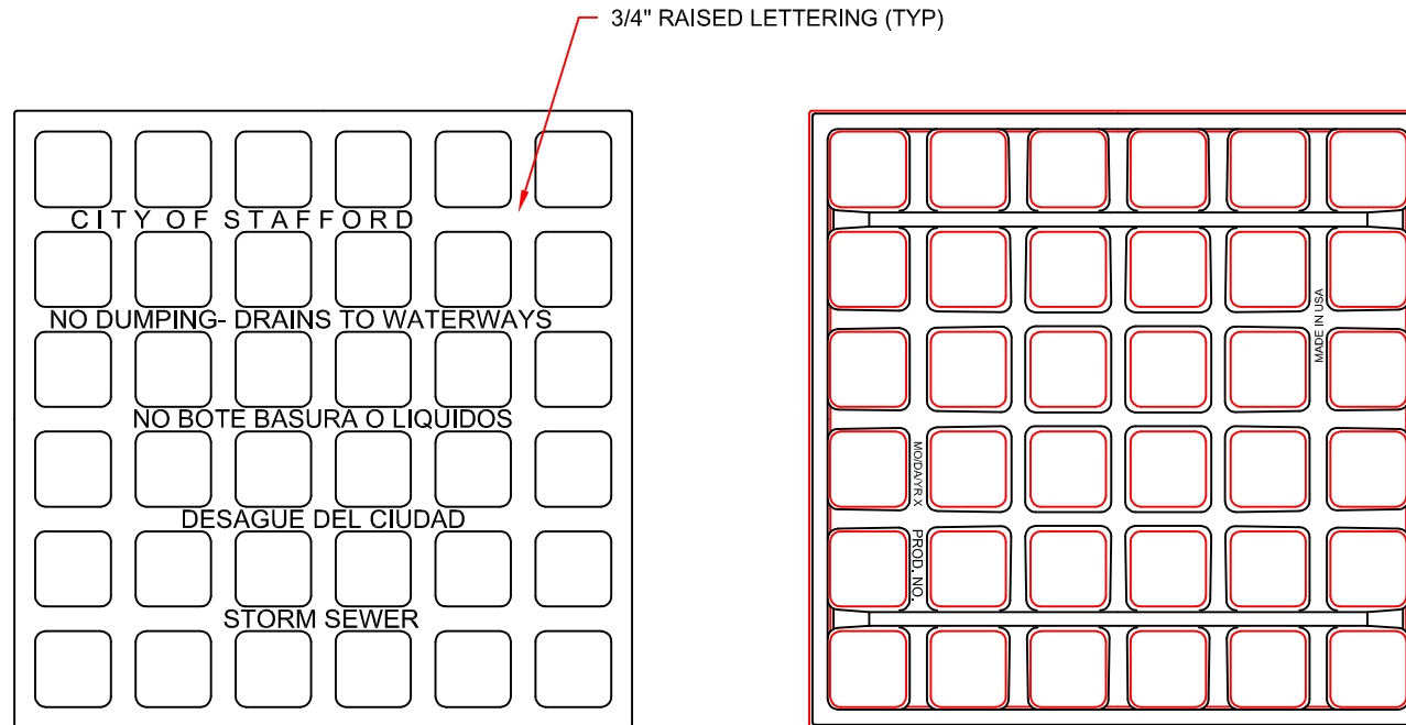
BOTTOM VIEW
